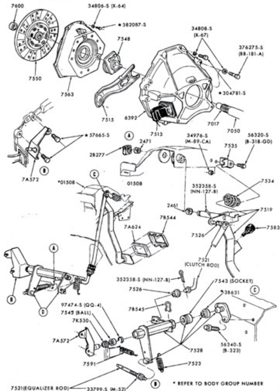
CLUTCH and CLUTCH PEDAL 1971/72 MUSTANG
